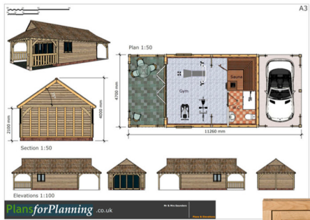
Planning Drawings
