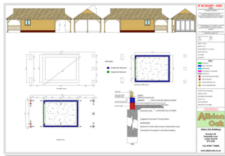
Groundworks Drawings
