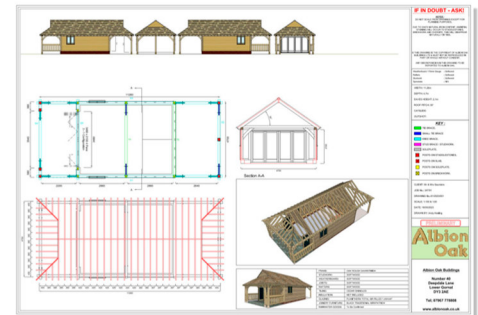
Frame Drawings
